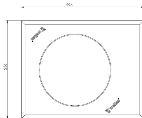
Dimensions of the cooktop (236 x 296 mm)
