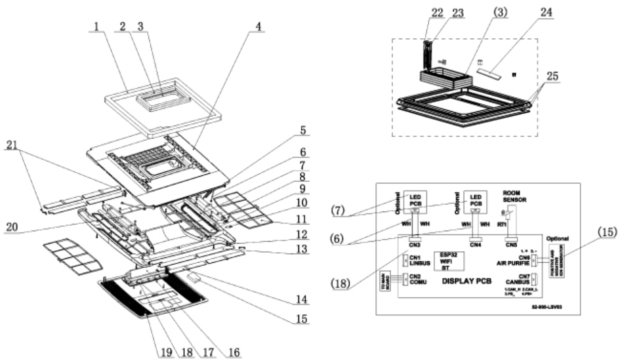
(Shape ADB Elec-906EM04_REV01)
